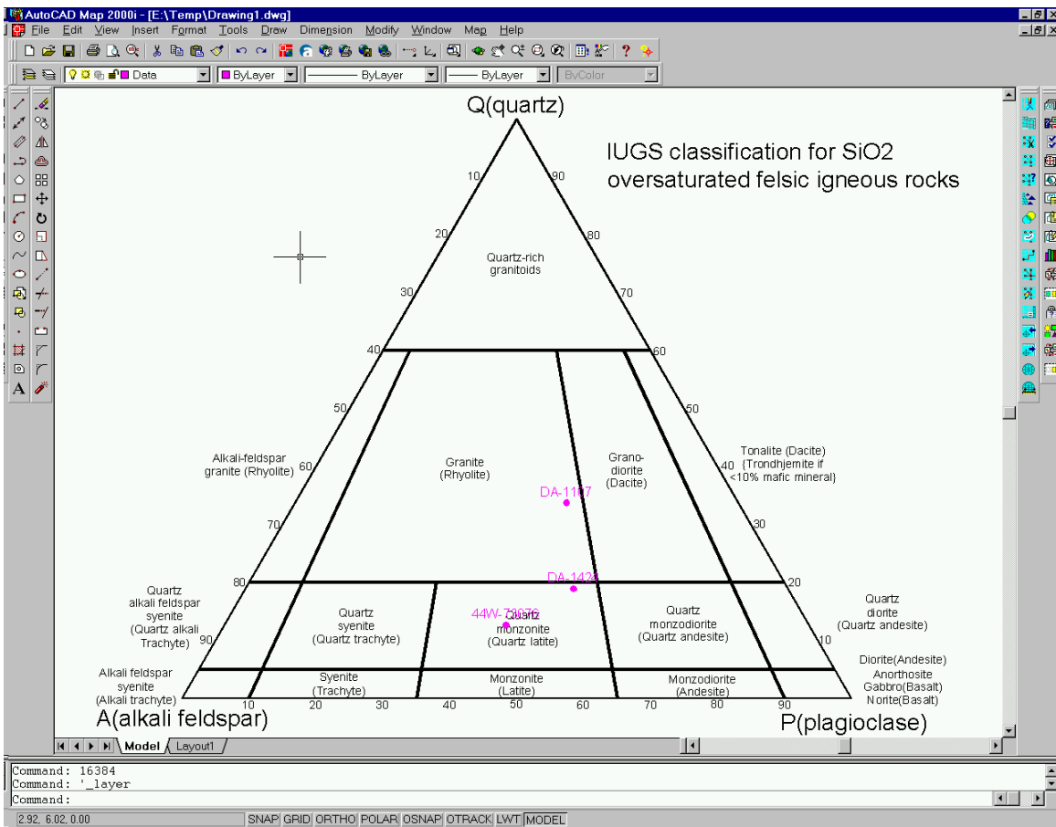
Figure 6: Triangular diagram with IUGS A-P-Q apices and data plotted.
