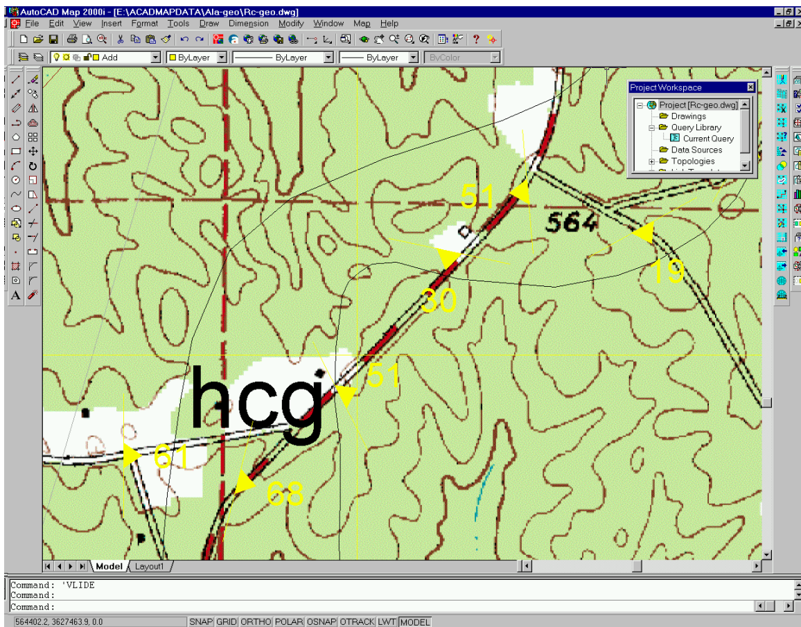
Figure 4: Structure data posted into the 1:24,000 geologic quadrangle base map with MAPPRO.
