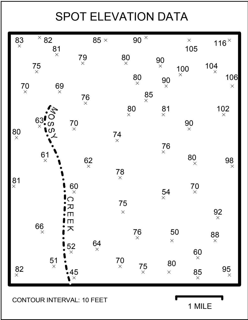
Figure 1. Spot elevations to be used for constructing topographic contours.
