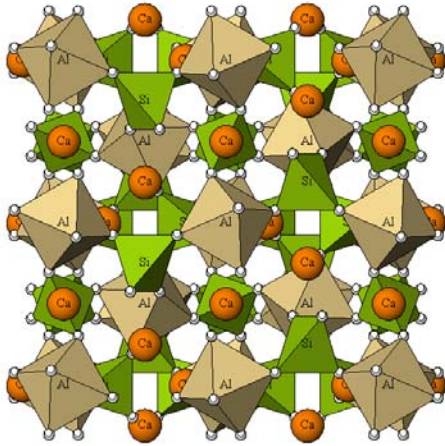
Structure of Grossular garnet
